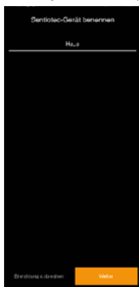
Fig. 8 Rename
