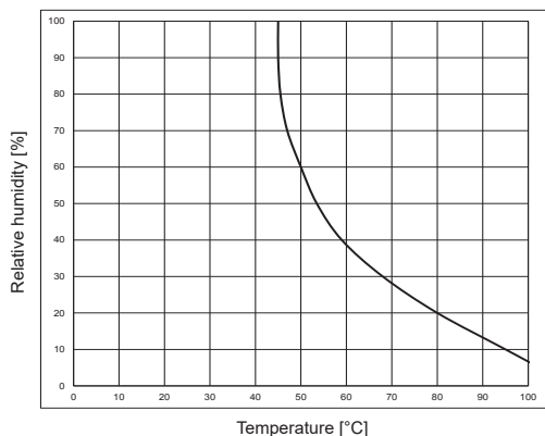
Fig. 7 Characteristic for temperature/relative humidity (compliant with EN 60335-2-53)
